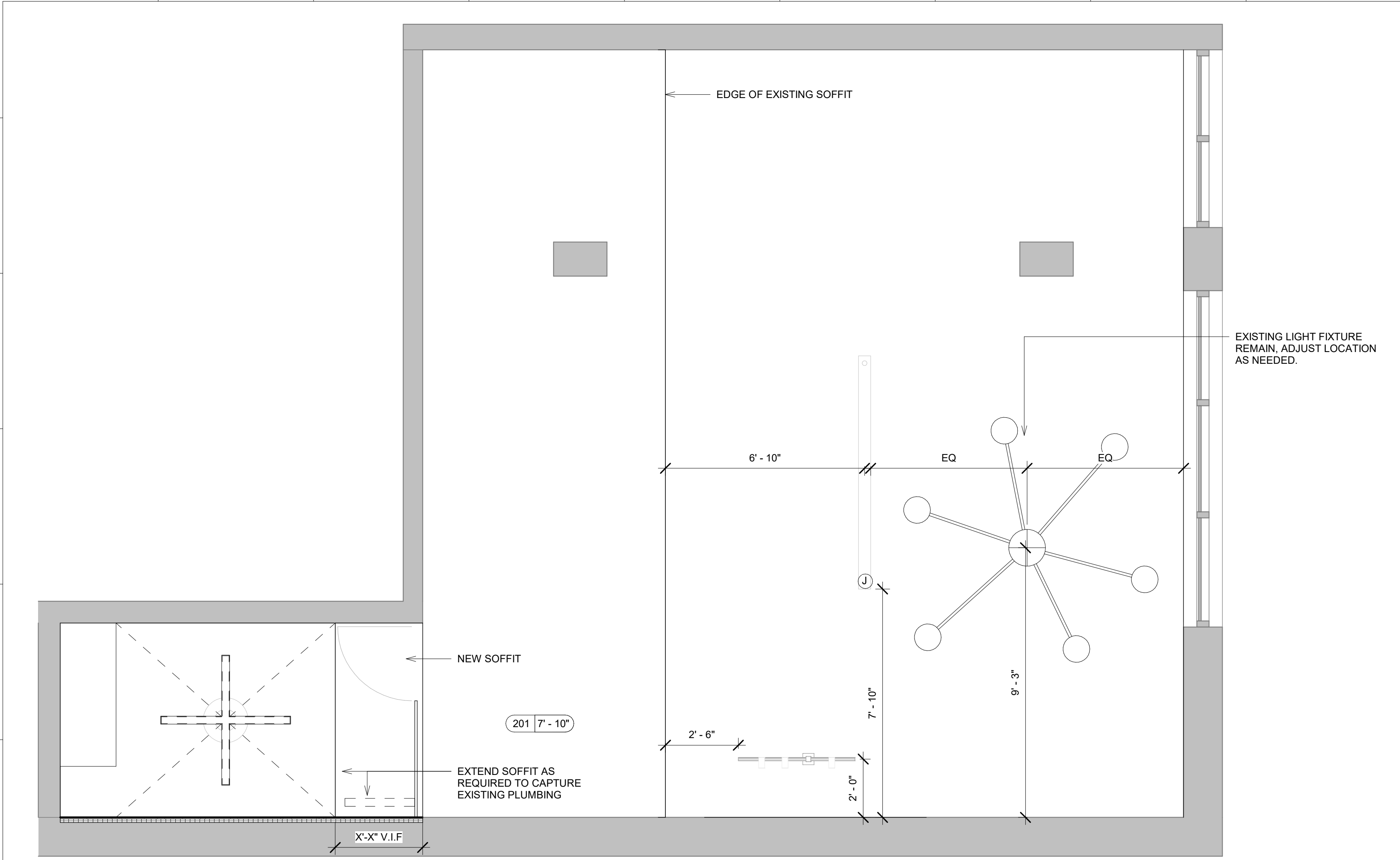
2 Level 2 3/8" = 1'-0"
