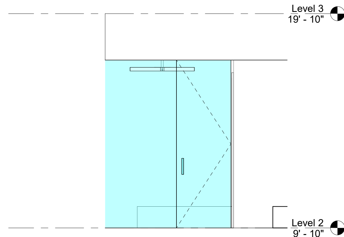
4 GLASS PARTITION 3/8" = 1'-0"
