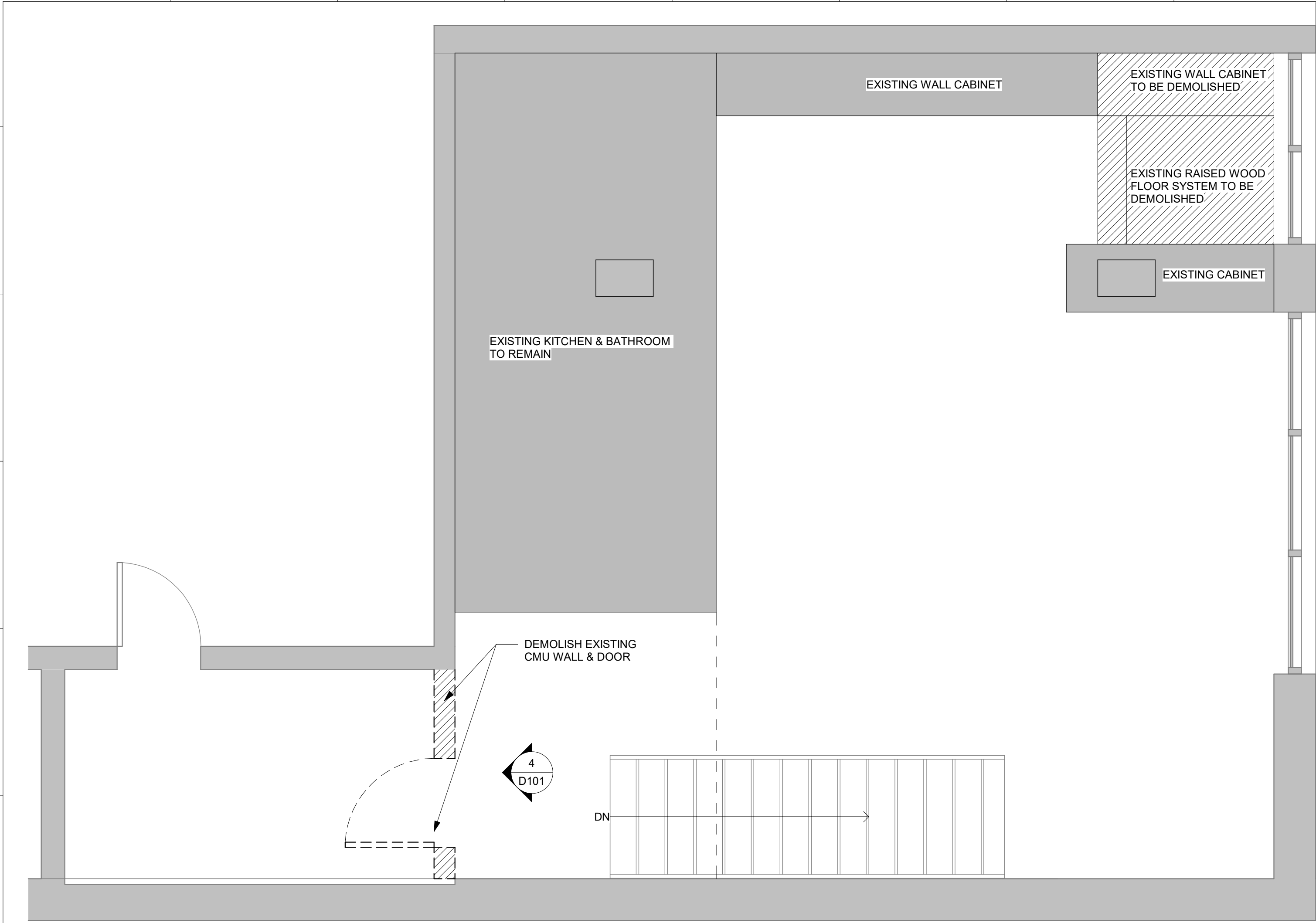
2 LEVEL 2 DEMO 3/8" = 1'-0"
