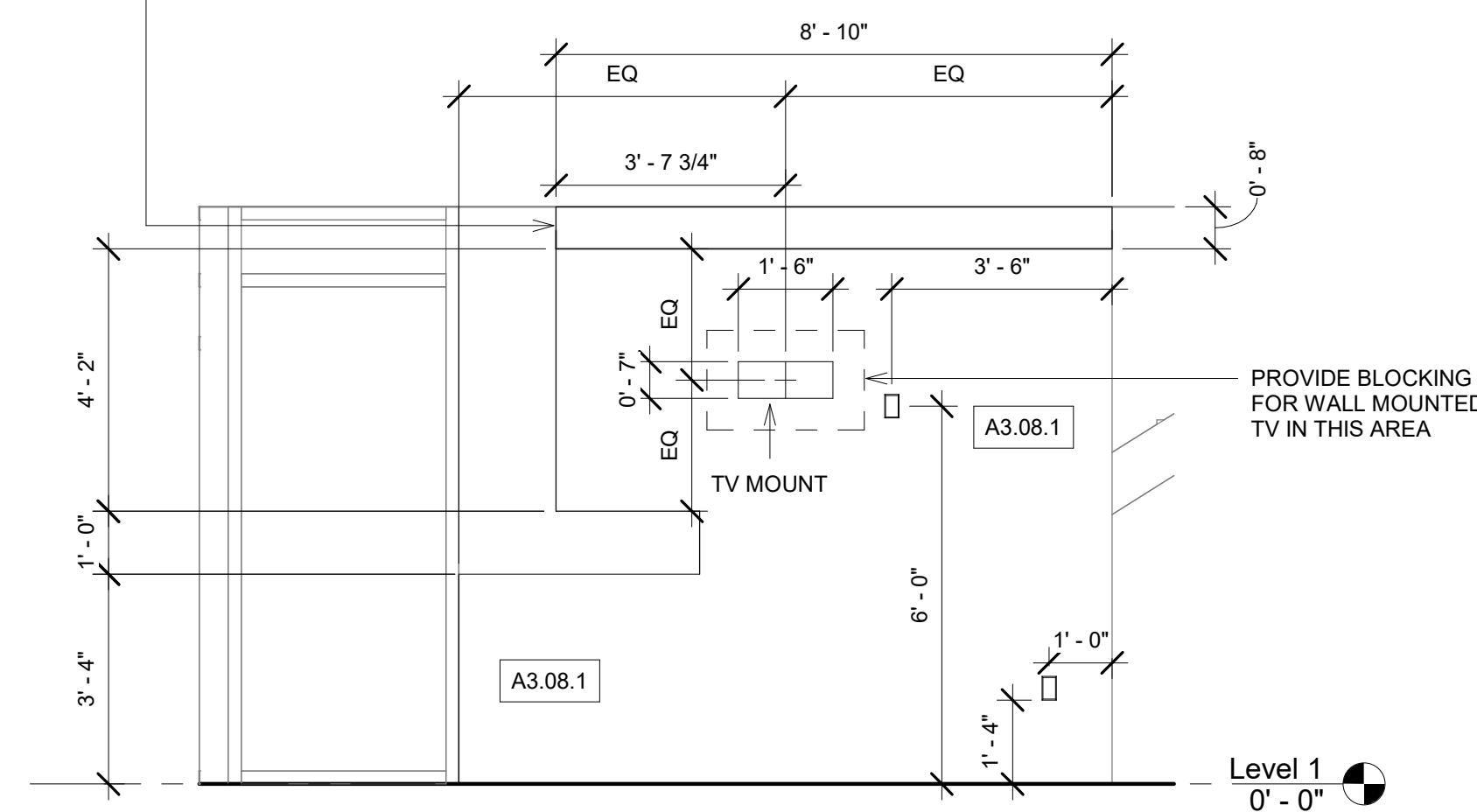
2 MEDIA WALL 3/8" = 1'-0"
